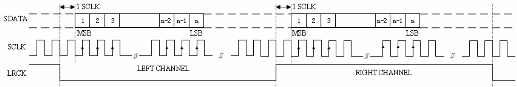
I 2 S Serial Audio Data Format Up To 24-bit
