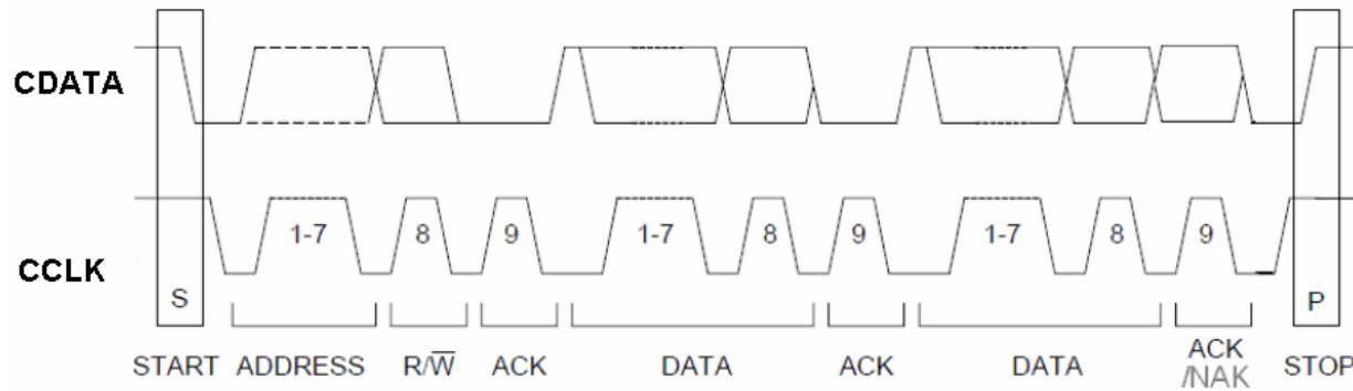
Figure 2. I2C timing
