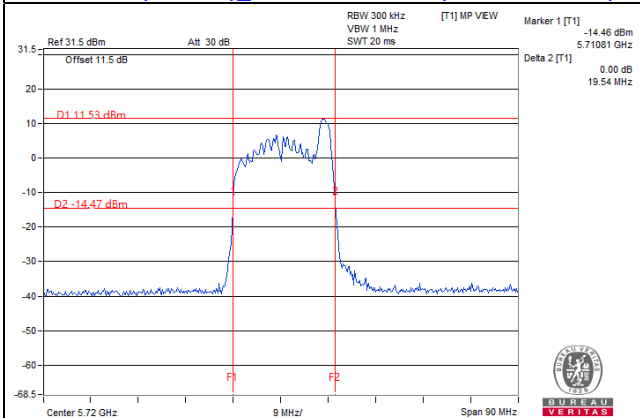
802.11ax (RU106/54)_Chain 1 / CH144 (U-NII-2C Band)
