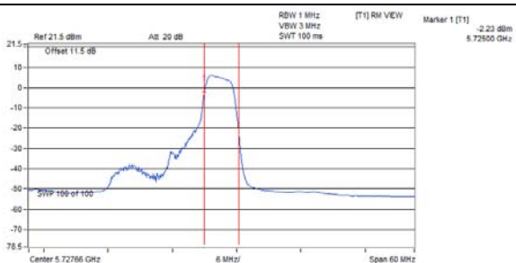
802.11ax (RU52/40)_Chain 1 / CH144 (U-NII-3 Band)
