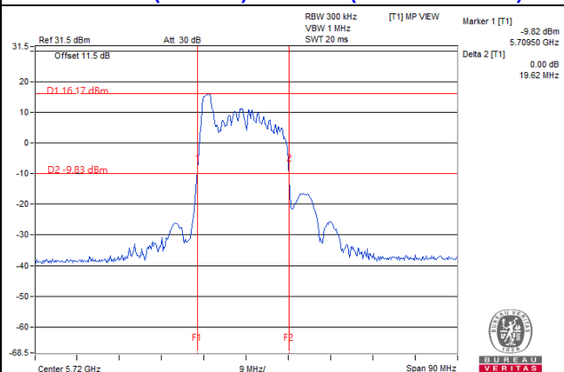
802.11ax (RU52/37) / CH144 (U-NII-2C Band)
