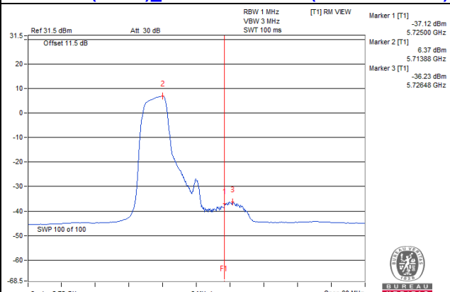
802.11ax (RU52)_Chain 0 / CH144 (U-NII-2C Band)
