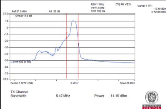
802.11ax (RU26/0) / CH144 (U-NII-3 Band)
