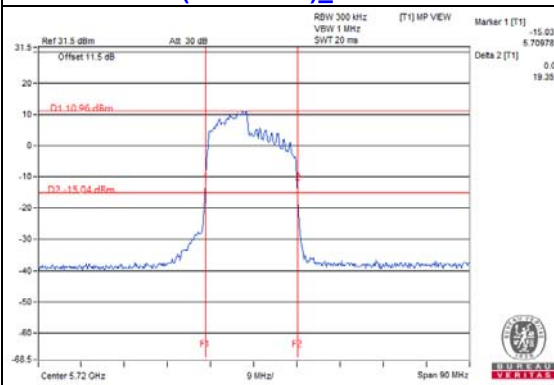
802.11ax (RU106/53)_Chain 0 / CH144
