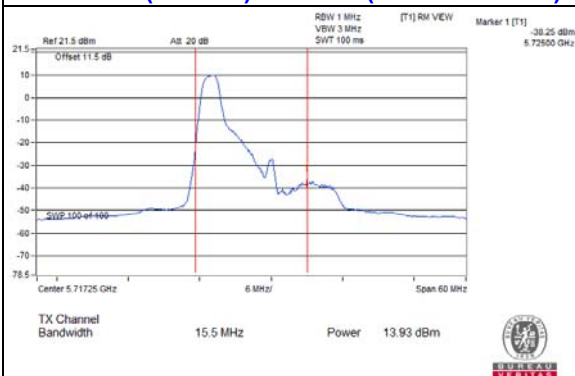
802.11ax (RU52/40) / CH144 (U-NII-2C Band)
