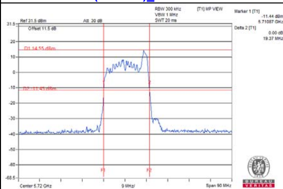
802.11ax (RU26/0)_Chain 1 / CH144
