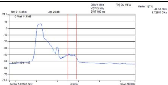
802.11ax (RU26/0)_Chain 1 / CH144 (U-NII-3 Band)
