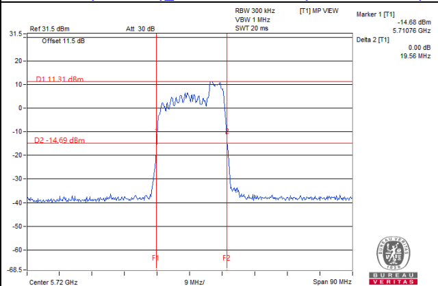
802.11ax (RU52/40)_Chain 1 / CH144 (U-NII-2C Band)
