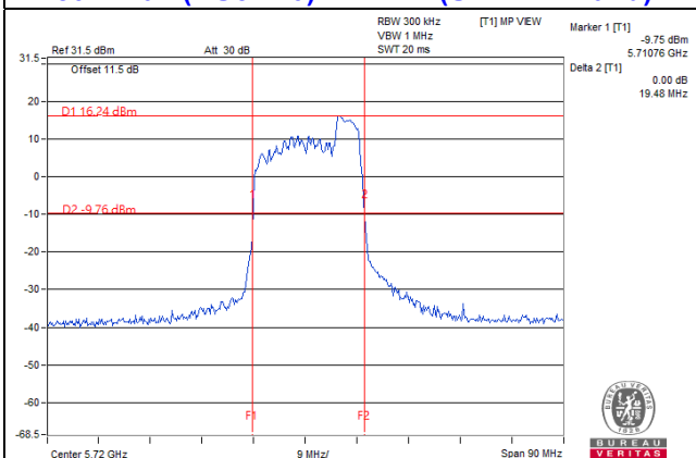
802.11ax (RU106/54) / CH144 (U-NII-2C Band)
