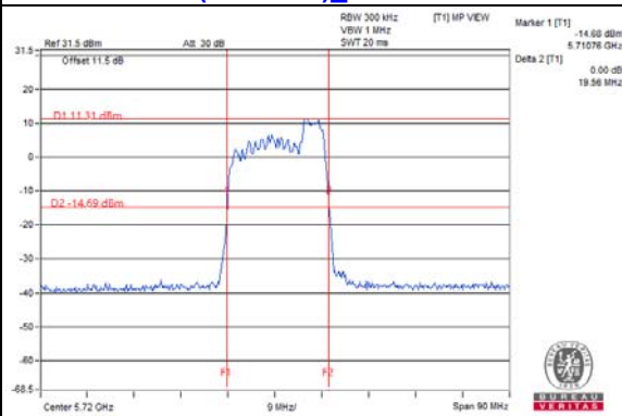
802.11ax (RU52/37)_Chain 1 / CH144
