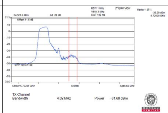
802.11ax (RU52/37)_Chain 1 / CH144 (U-NII-3 Band)
