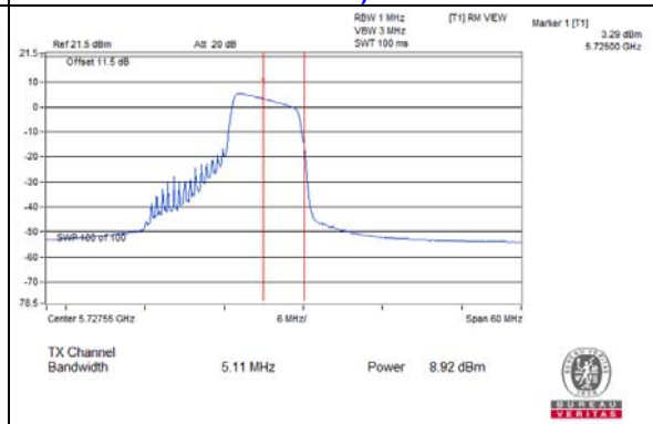
802.11ax (RU106/54)_Chain 1 / CH144 (U-NII-3 Band)
