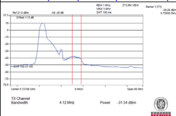
802.11ax (RU52/40) / CH144 (U-NII-3 Band)
