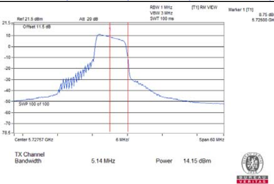
802.11ax (RU106/53) / CH144 (U-NII-3 Band)
