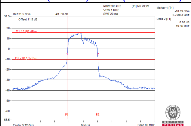
802.11ax (RU106/53) / CH144 (U-NII-2C Band)
