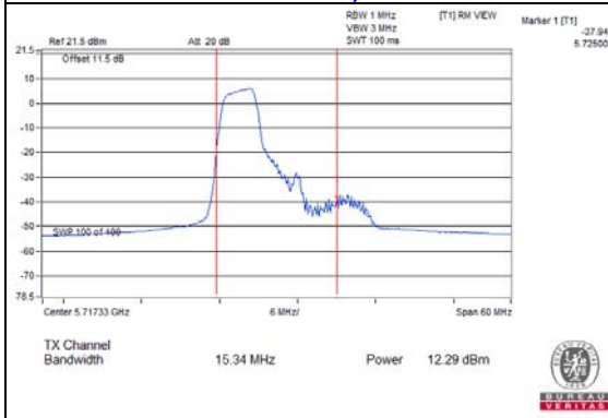
802.11ax (RU106/54)_Chain 0 / CH144 (U-NII-2C Band)
