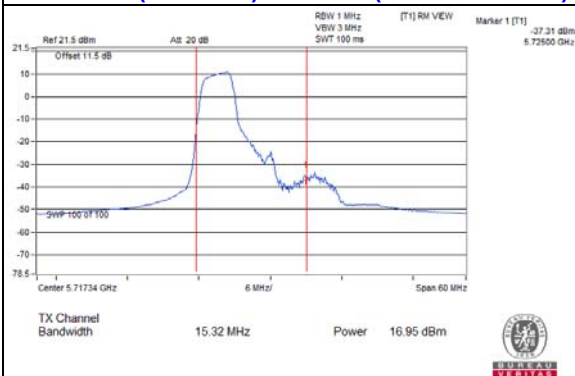
802.11ax (RU52/37) / CH144 (U-NII-2C Band)
