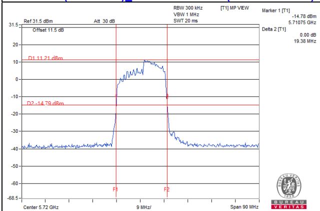
802.11ax (RU106/54)_Chain 1 / CH144 (U-NII-2C Band)
