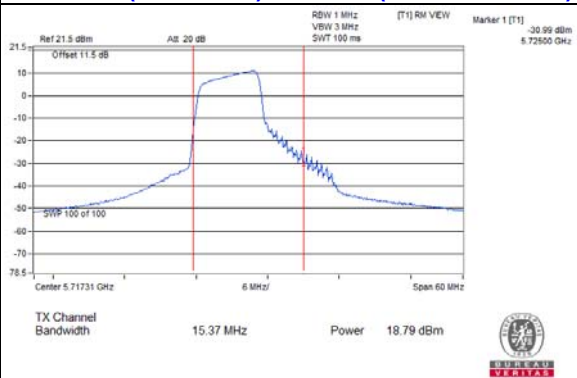
802.11ax (RU106/53) / CH144 (U-NII-2C Band)
