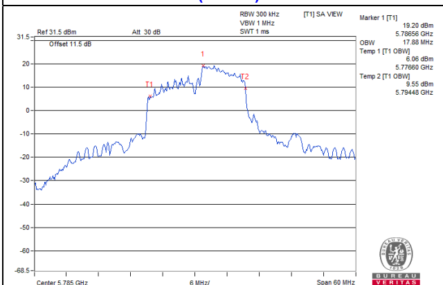
802.11ax (RU106) / CH157
