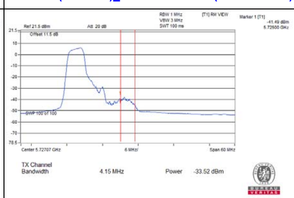
802.11ax (RU106/54)_Chain 0 / CH144 (U-NII-3 Band)
