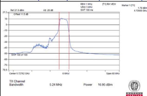
802.11ax (RU52/37) / CH144 (U-NII-3 Band)
