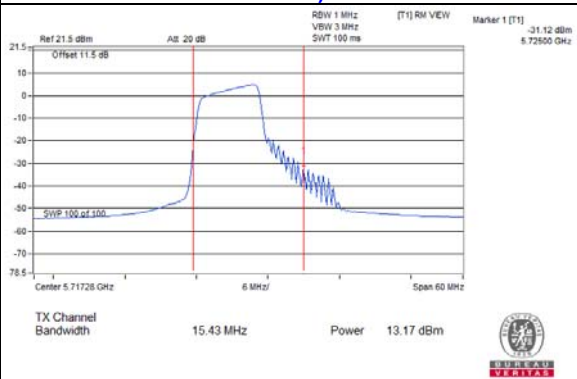
802.11ax (RU106/53)_Chain 1 / CH144 (U-NII-2C Band)
