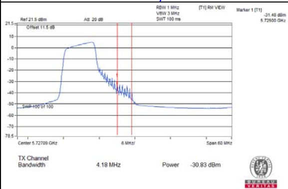
802.11ax (RU106/53)_Chain 1 / CH144 (U-NII-3 Band)
