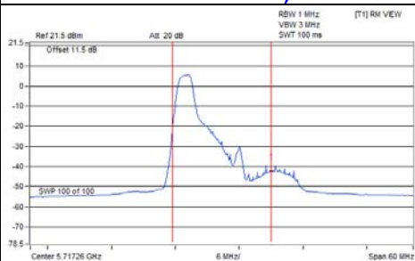
802.11ax (RU26/0)_Chain 0 / CH144 (U-NII-2C Band)
