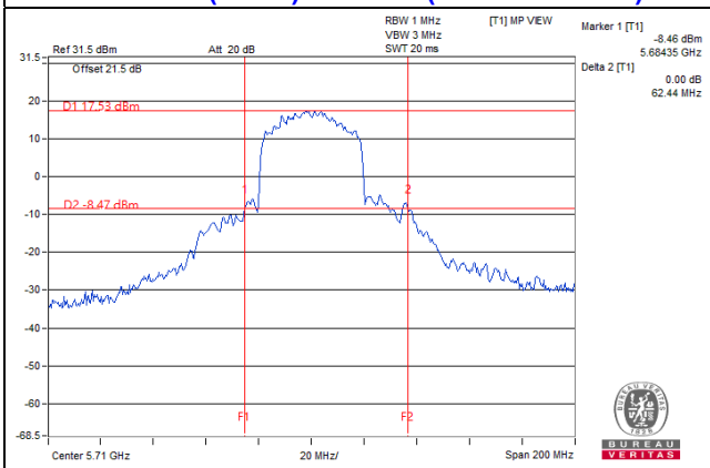
802.11ax (HE40) / CH142 (U-NII-2C Band)
