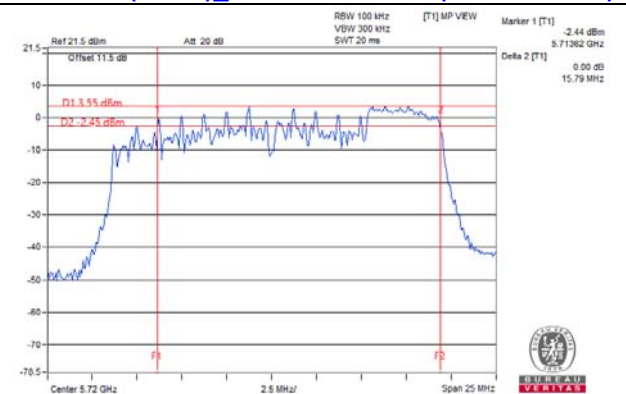
802.11ax (RU52)_Chain 0 / CH144 (U-NII-3 Band)
