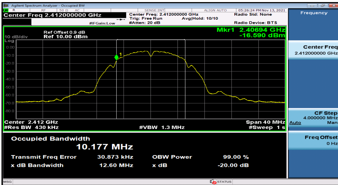
Test Plots 802.11b: Low Channel
