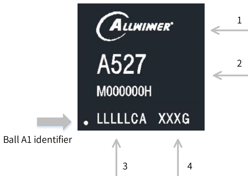
Figure 12-4 A527M000000H Marking
