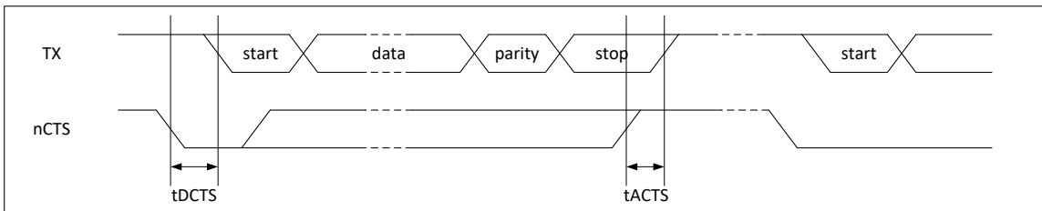
Figure 6-24 UART nRTS Timing
