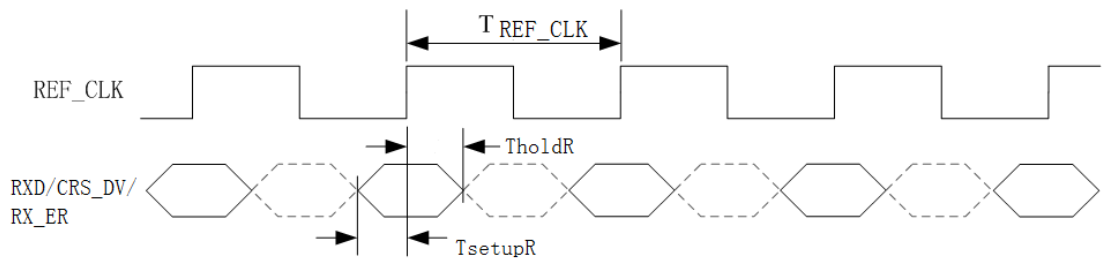
Figure 6-35 RMII Transmit Timing
