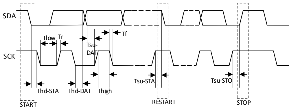
Figure 6-31 TWI Timing
