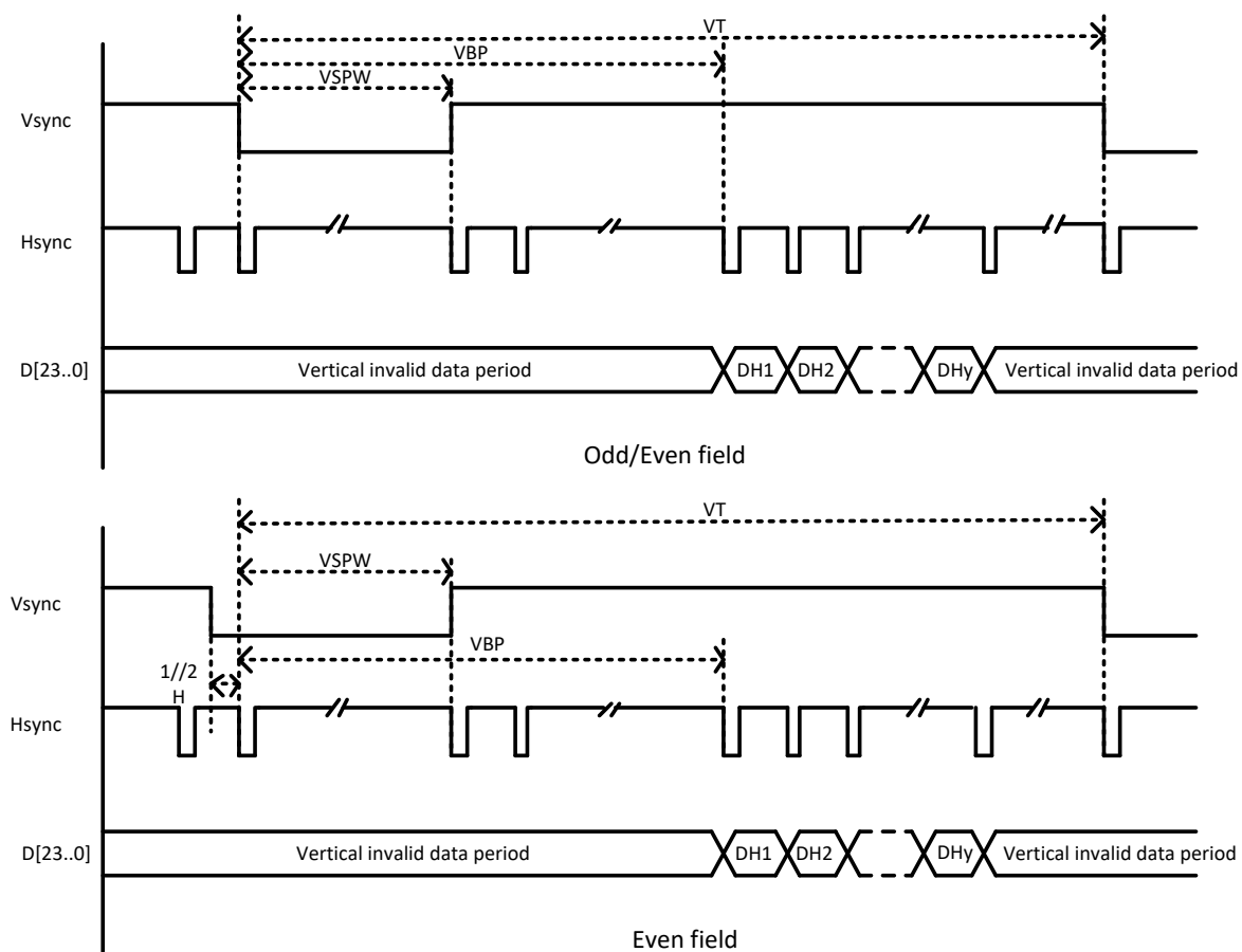
Figure 6-40 HV_IF Vertical Timing
