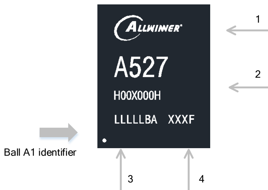
Figure 12-2 A527H00X000H Marking
