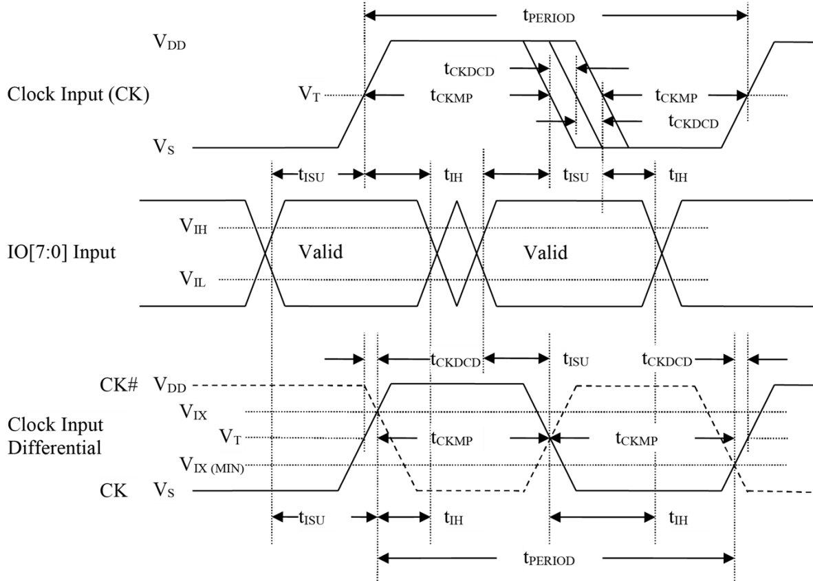
Figure 6-29 xSPI Target Data Input Timing
