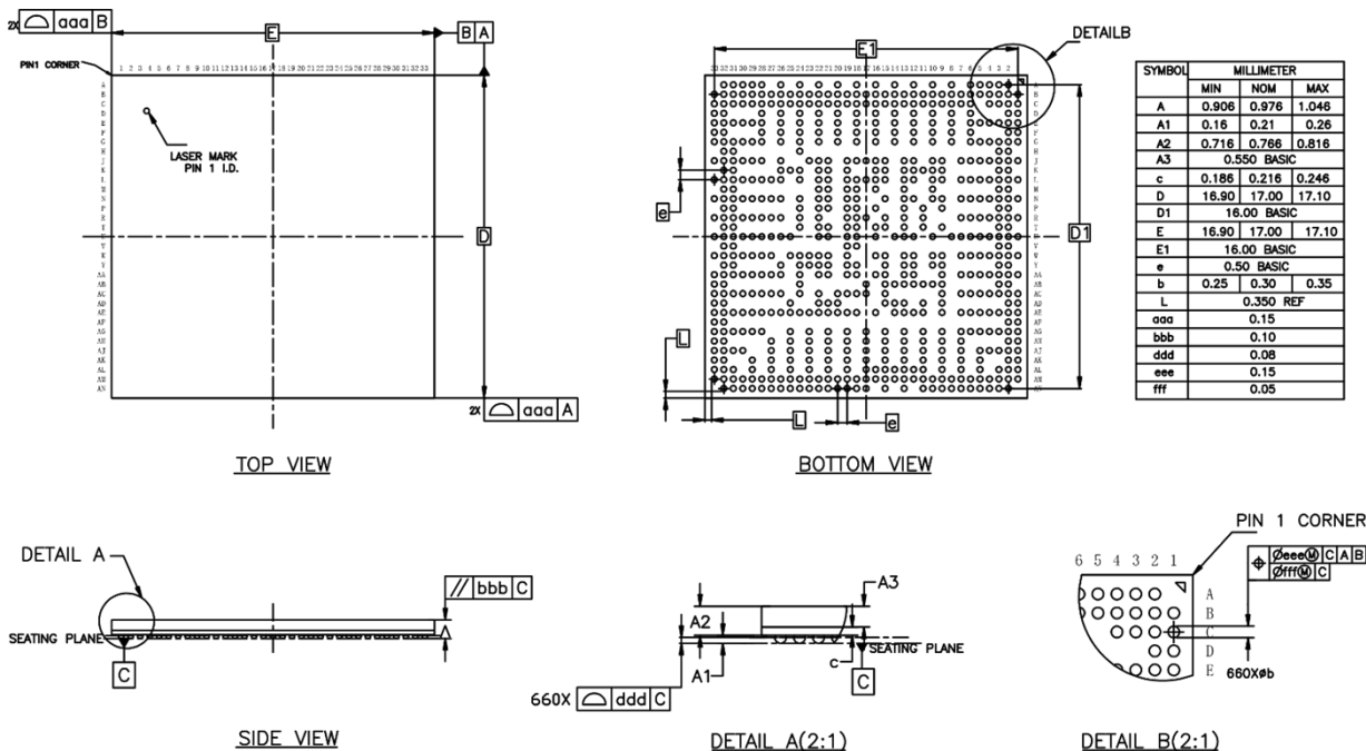
Figure 8-3 Package Dimension
