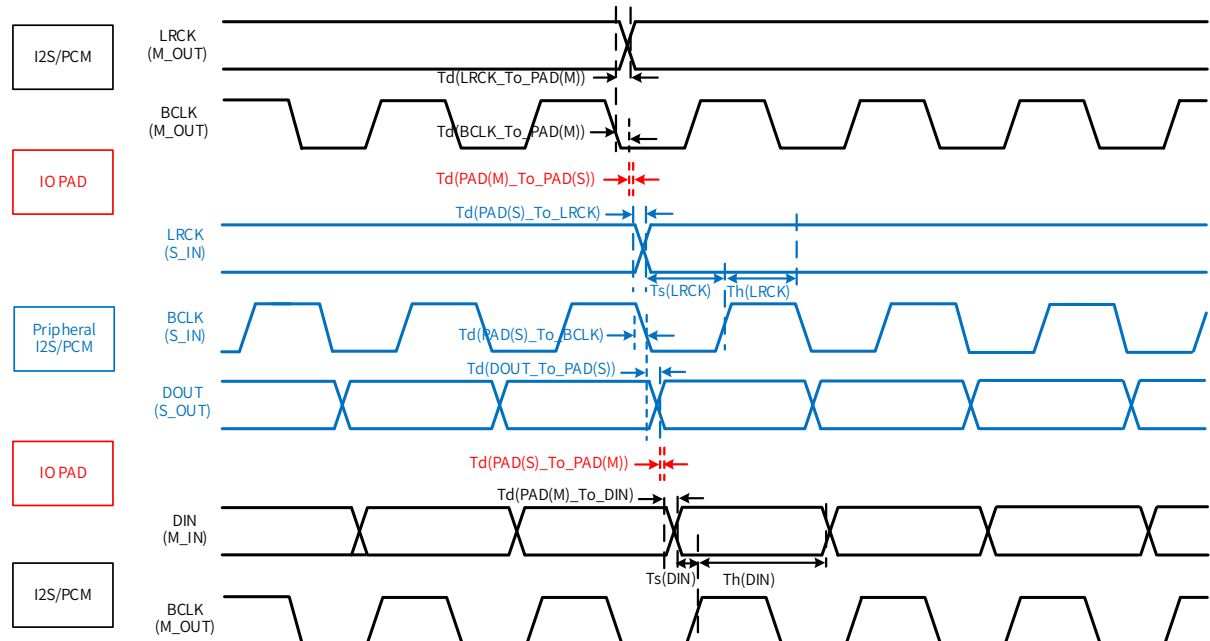
Figure 6-45 Data Input Timing of I2S/PCM in Master Mode
