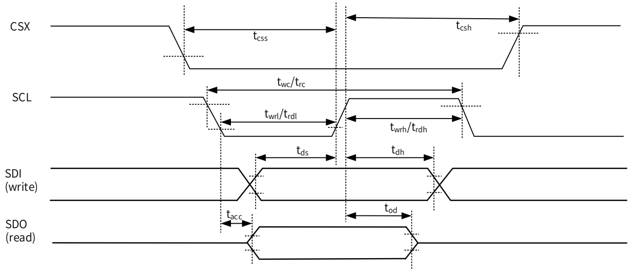
Figure 6-27 DBI 3-line Serial Interface Timing
