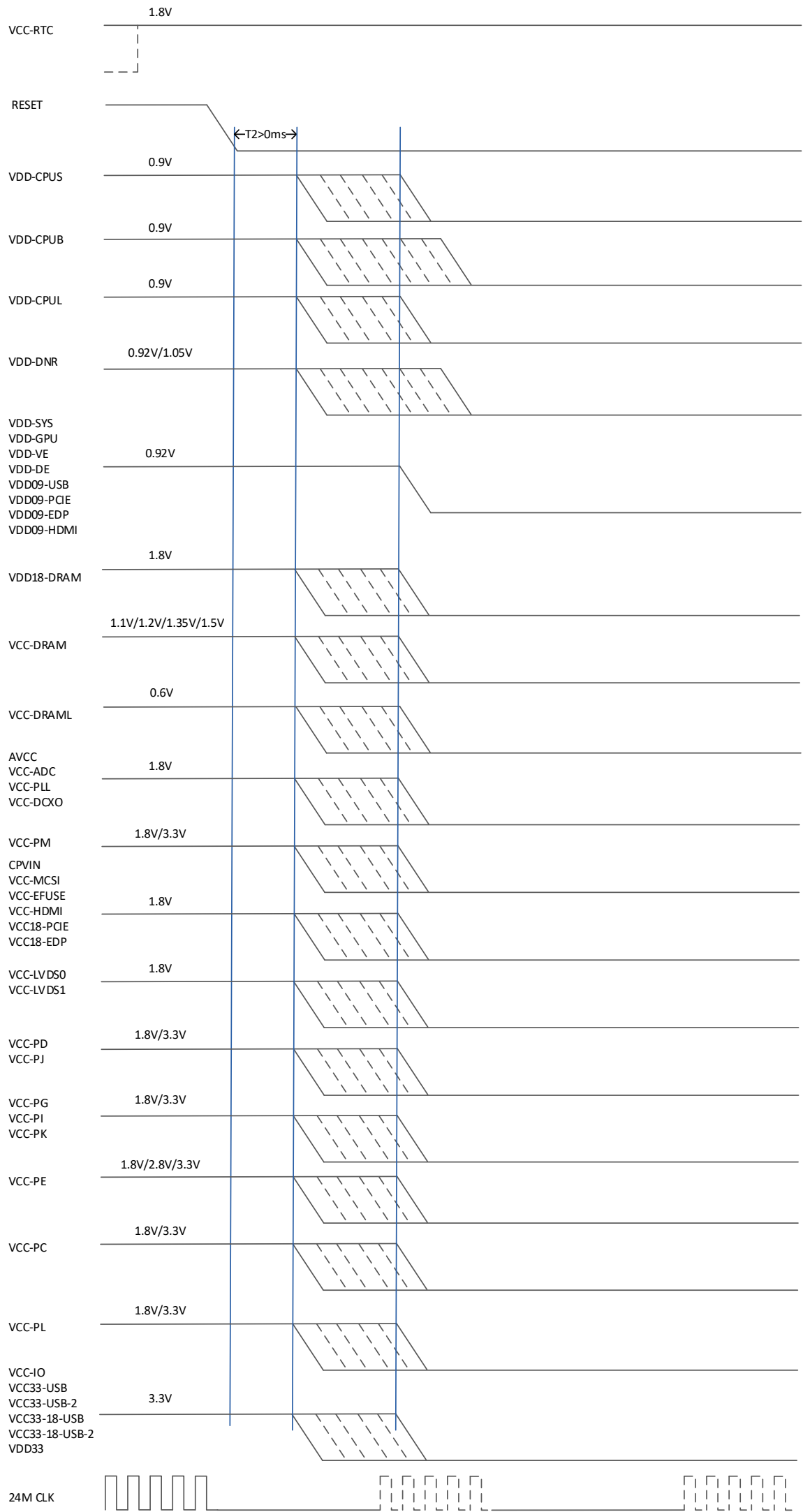
Figure 6-48 Power-off Timing
