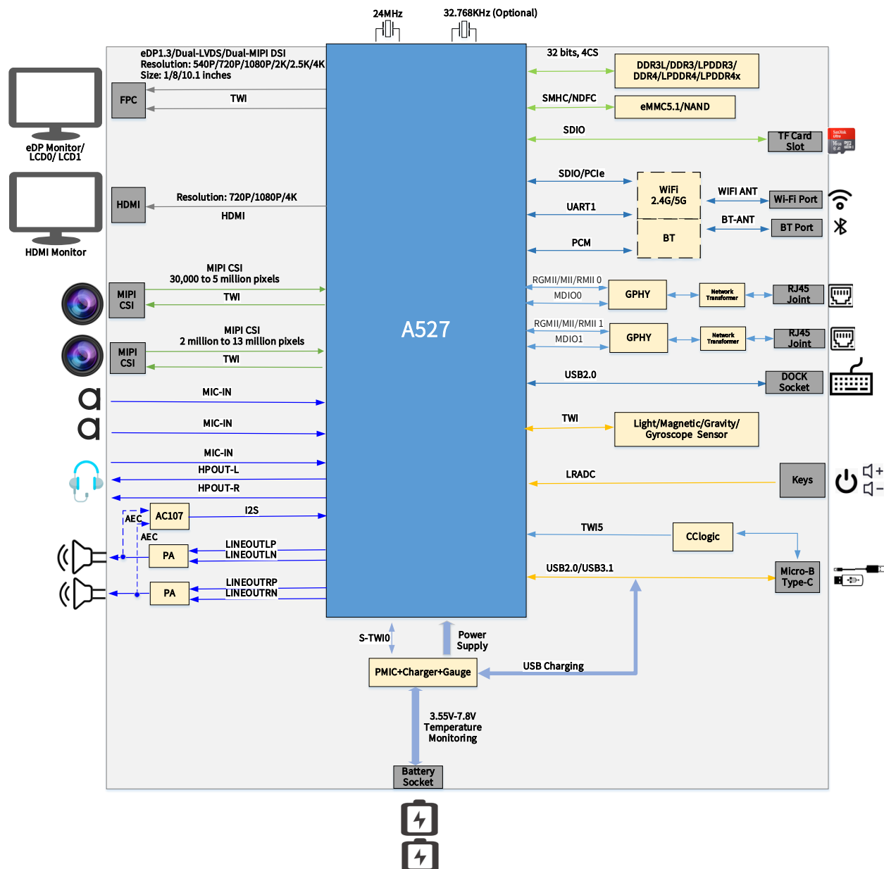
Figure 4-2 ARM PC Solution
