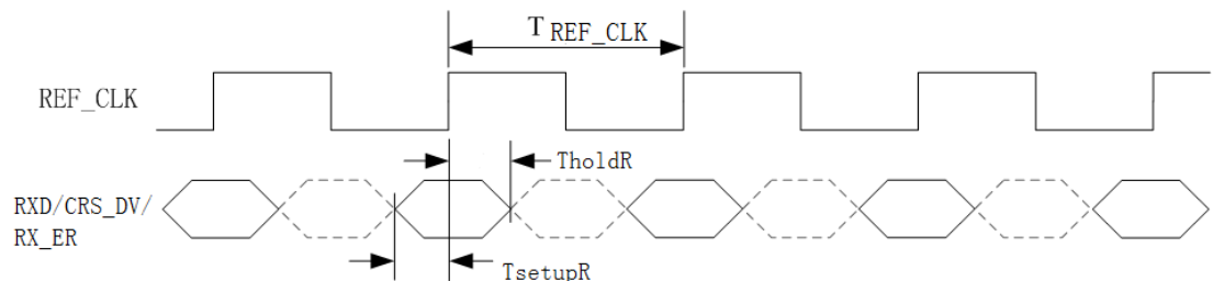
Figure 6-39 RMII Transmit Timing
