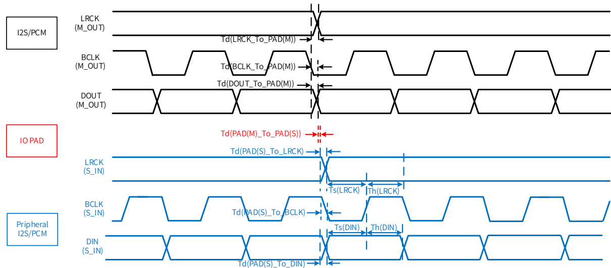
Figure 6-44 Data Output Timing of I2S/PCM in Master Mode
