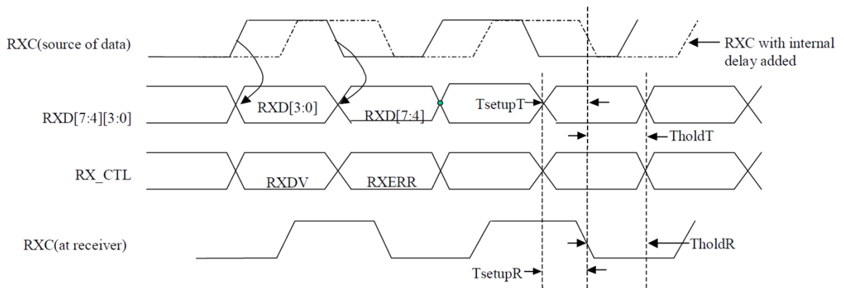
Figure 6-33 RGMII Transmit Timing
