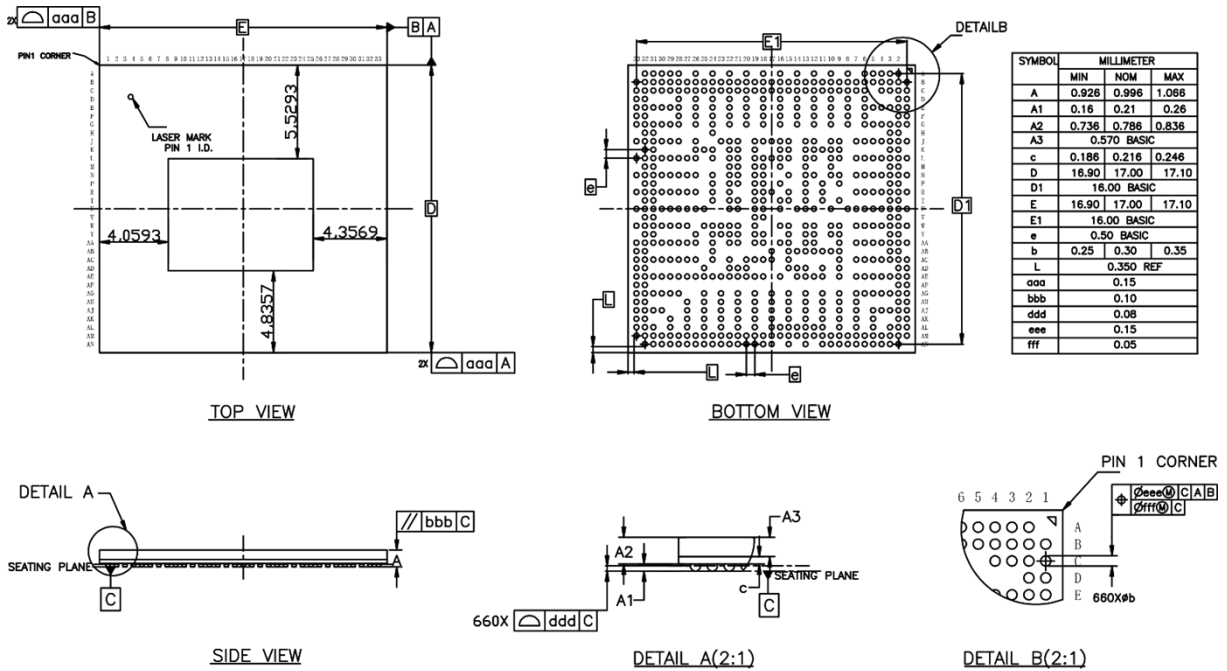
Figure 8-2 Package Dimension
