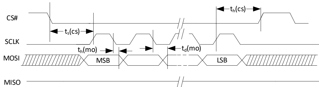
Figure 6-25 SPI Writing Timing
