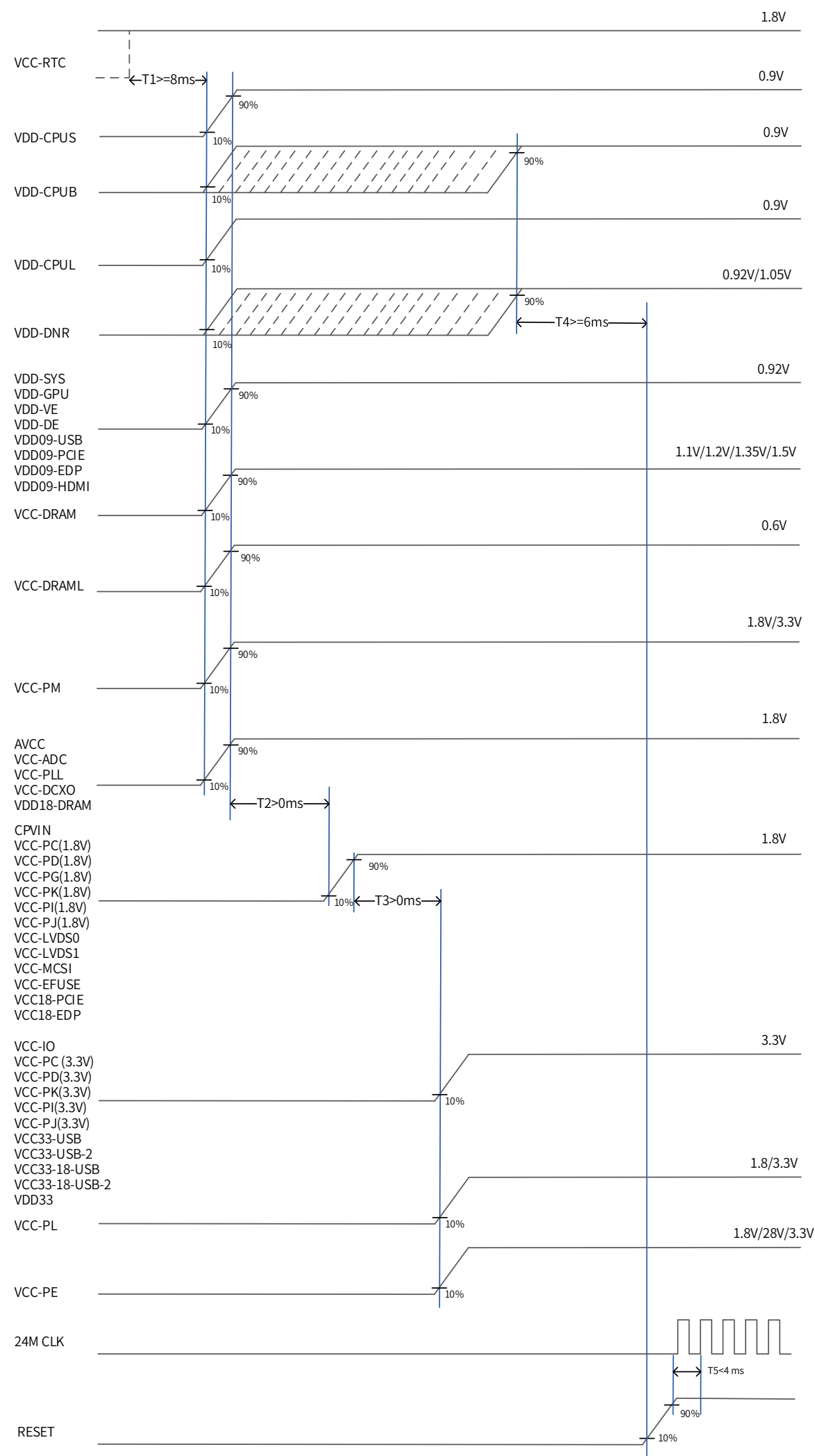
Figure 6-47 Power-on Timing
