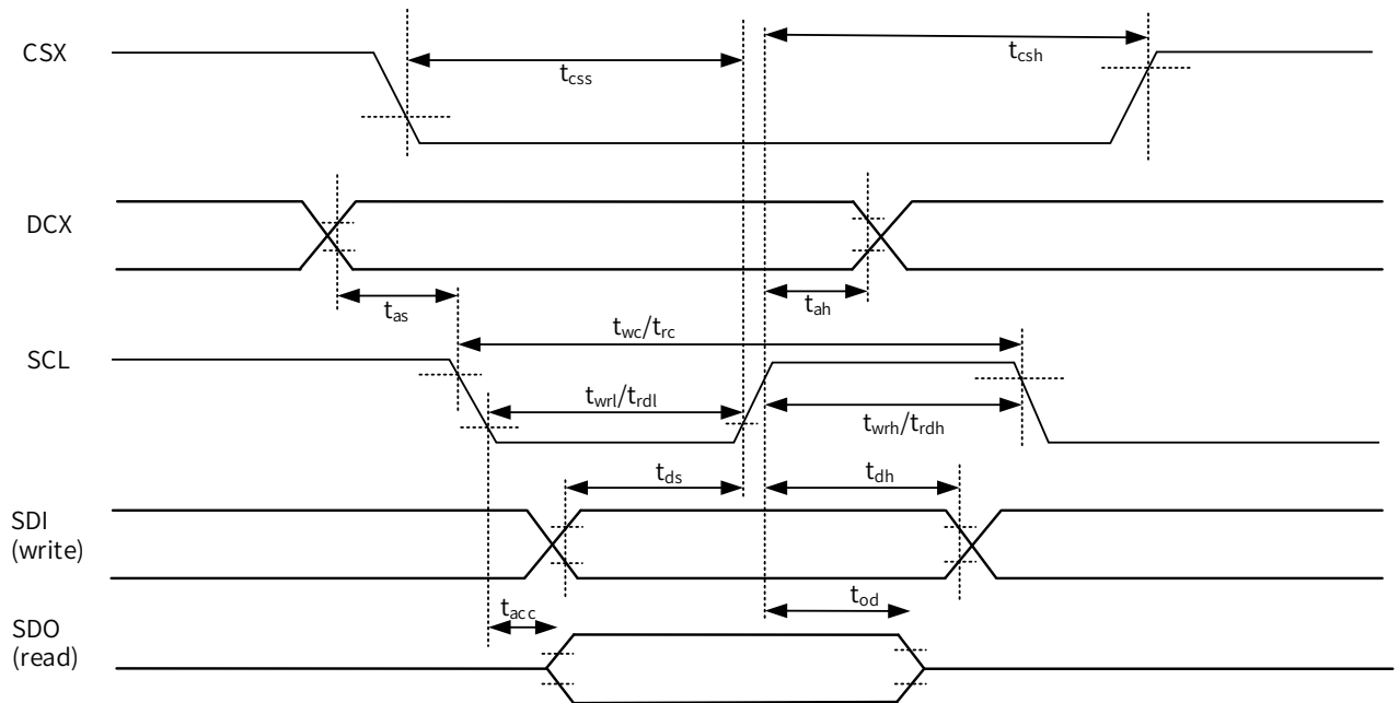
Figure 6-28 DBI 4-line Serial Interface Timing
