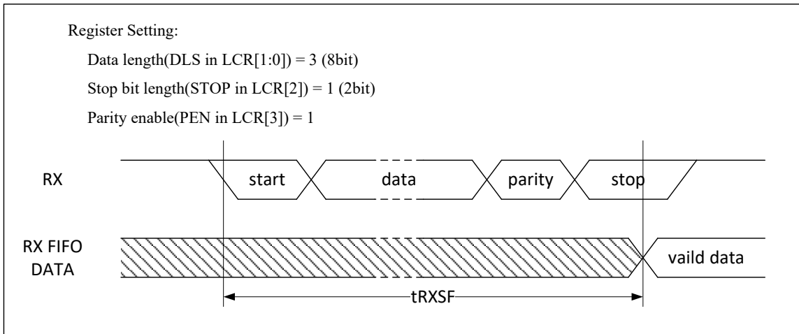
Figure 6-23 UART nCTS Timing
