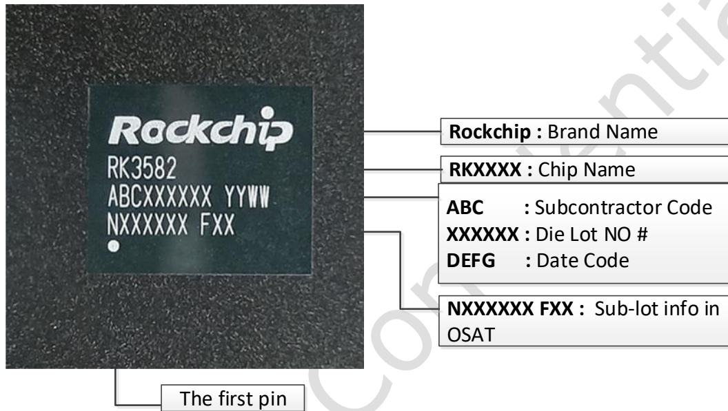
Fig.2-1 Package definition
