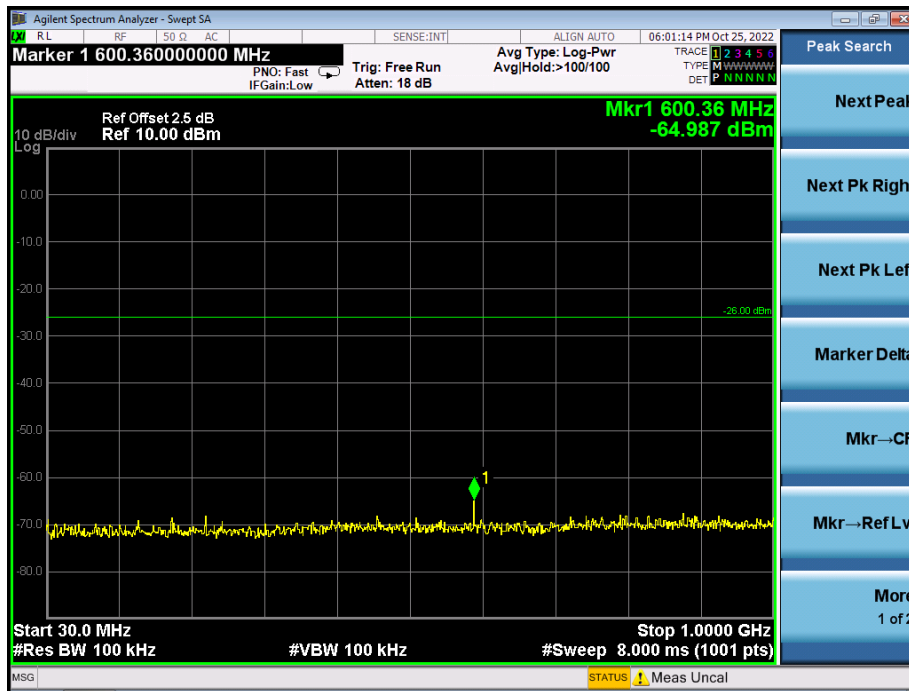
CH 00- Frequency Band 1 (30 MHz ≤ f ≤ 1000 MHz)
