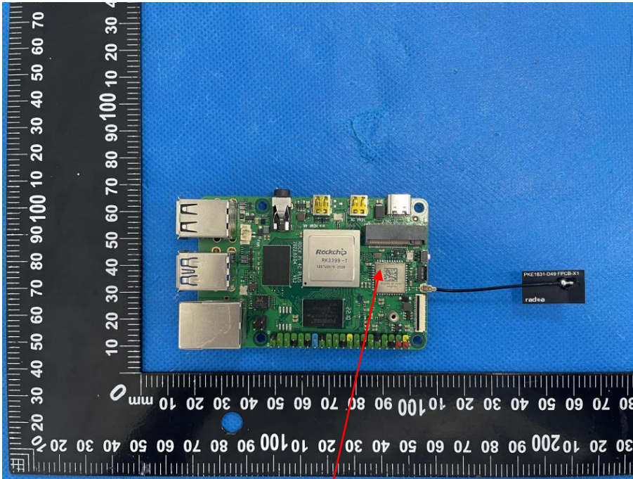
Built-in shielding cover
