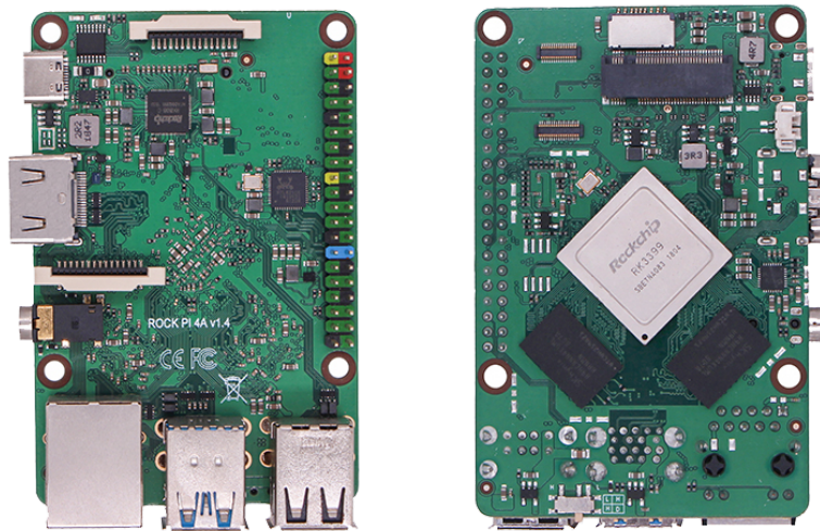
Figure 1: Radxa ROCK 4B
