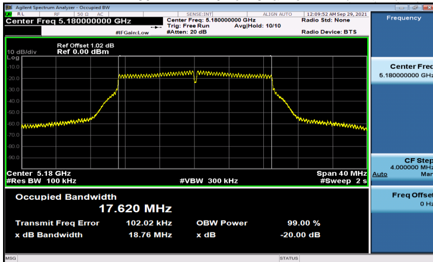
802.11n HT20 Low Channel
