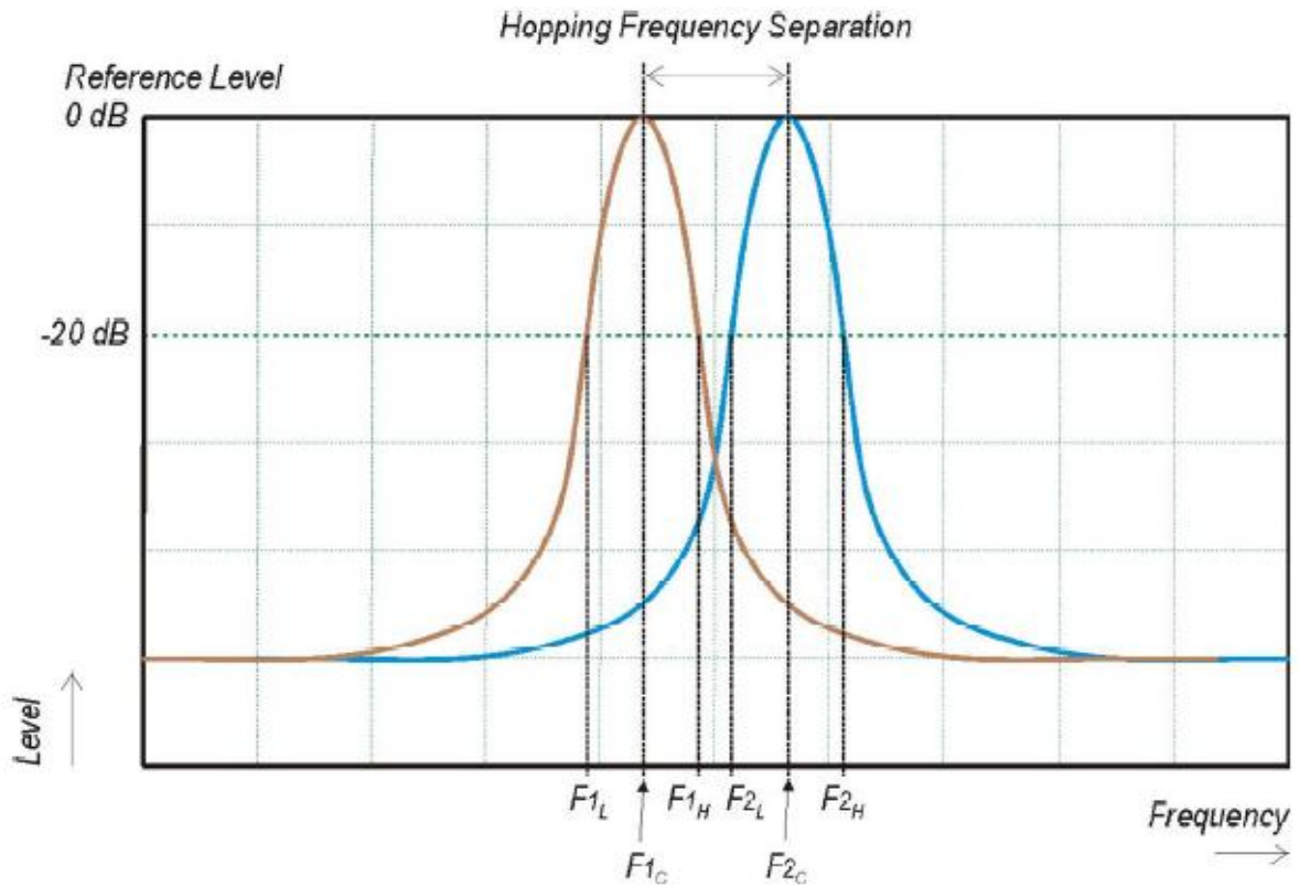
Figure 4: Hopping Frequency Separation
