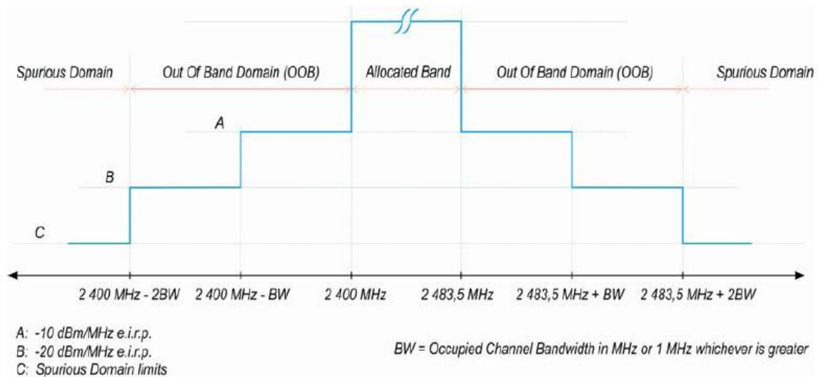
Figure 3: Transmit mask
