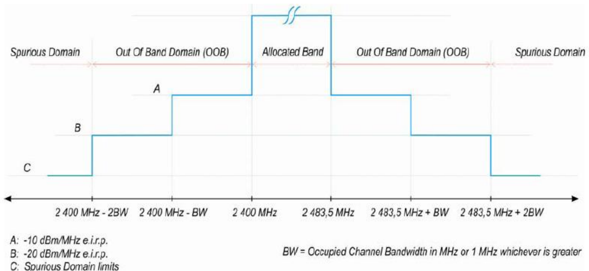
Figure 3: Transmit mask
