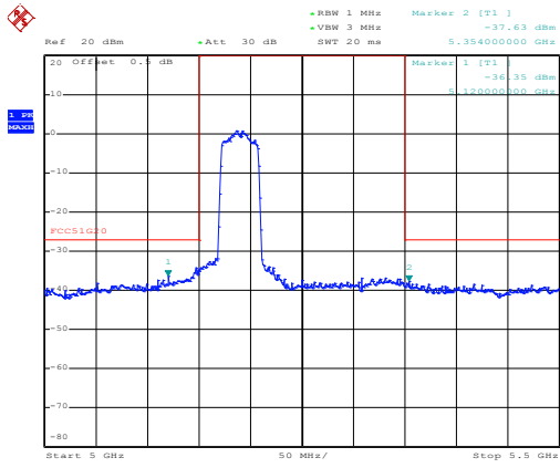
(802.11n40) Band Edge, Left Side
