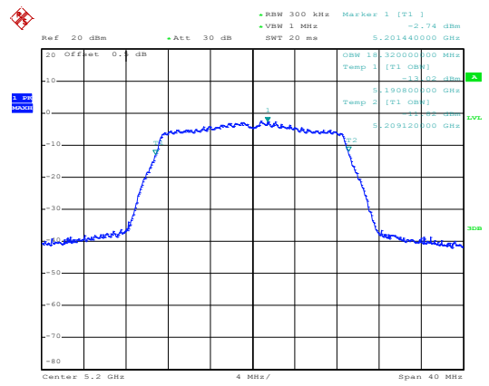
(802.11 AC20) 99%Bandwidth plot on channel 40
