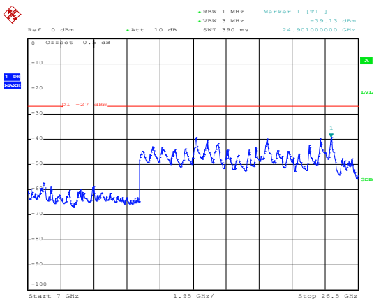
802.11 ac40 on channel 46
