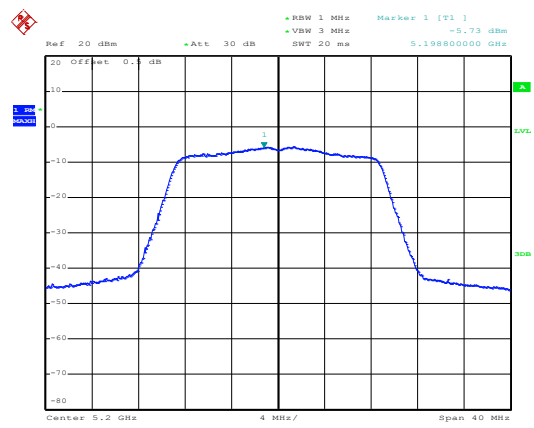
(802.11ac20) PSD plot on channel 40
