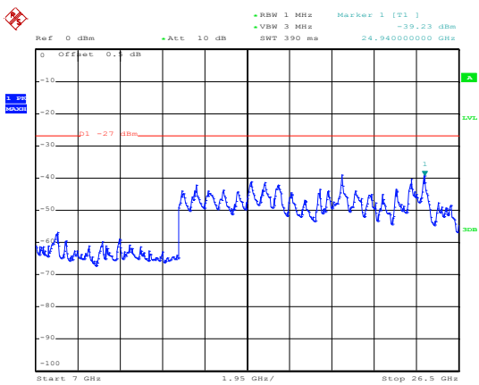
802.11n40 on channel 38
