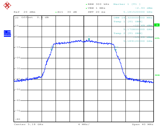
(802.11 AC20) 99%Bandwidth plot on channel 36
