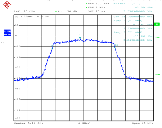
(802.11 AC20) 99%Bandwidth plot on channel 48
