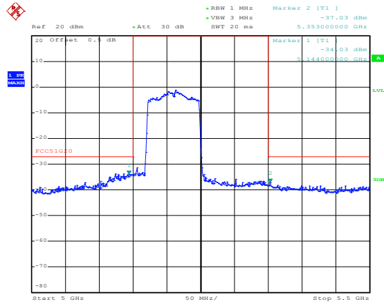
(802.11ac80) Band Edge, Left Side
