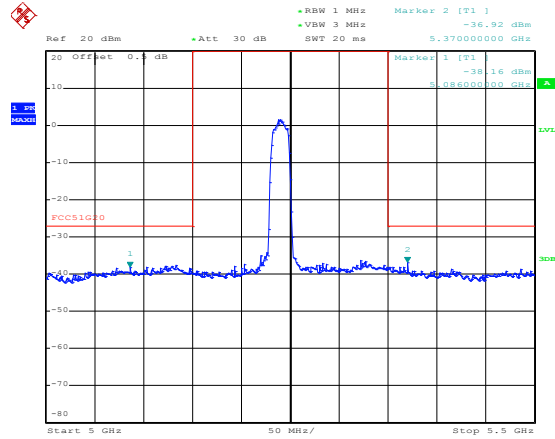
(802.11ac20) Band Edge, Right Side
