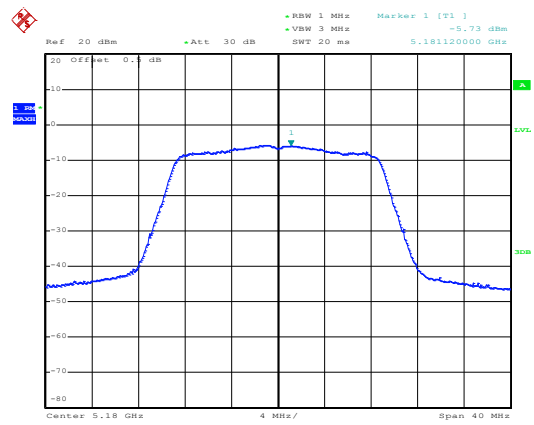
(802.11ac20) PSD plot on channel 36
