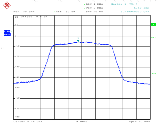
(802.11ac20) PSD plot on channel 48
