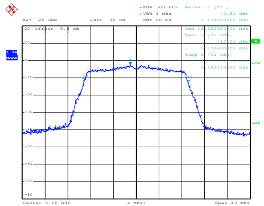
(802.11 n20) 99%Bandwidth plot on channel 36
