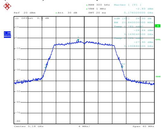
(802.11 AC20) -26dB Bandwidth plot on channel 38
