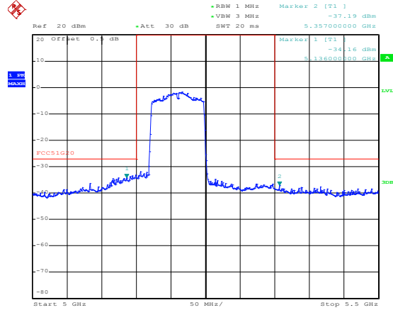
(802.11ac80) Band Edge, Right Side
