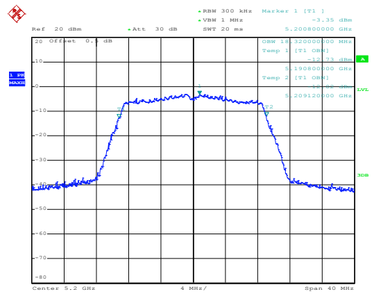
(802.11 n20) 99%Bandwidth plot on channel 40
