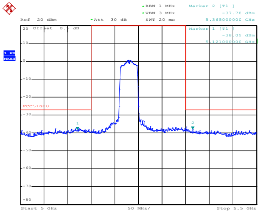
(802.11ac40) Band Edge, Right Side
