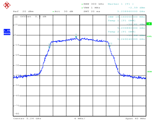
(802.11 AC80) 99%Bandwidth plot on channel 42
