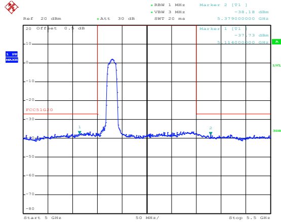
(802.11ac20) Band Edge, Left Side
