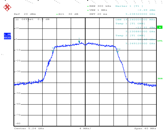
(802.11 n20) 99%Bandwidth plot on channel 48
